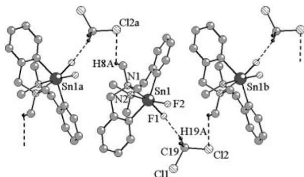
Figure 3. Polymeric associations in the crystal of compound 1b ·CH 2 Cl 2 based on halogen-hydrogen contacts (only hydrogens involved in such contacts are shown) [symmetry-equivalent atoms ( x, 2 - y, 0.5 + z ) and ( x, 2 - y, -0.5 + z ) are labelled as “a” and “b”].
