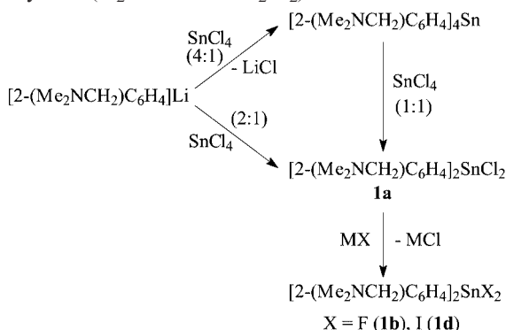
Scheme 1. Synthesis of compounds 1a–1d .
