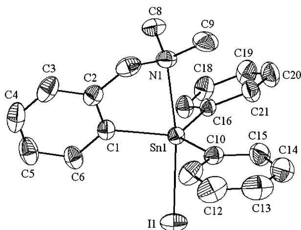
Figure 2. ORTEP representation at 30% probability and atom-numbering scheme for the isomer ( S )- 3d . Hydrogens have been omitted for clarity.
