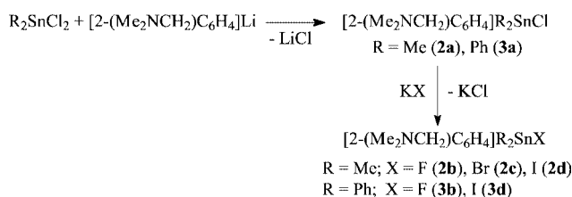
Scheme 2. Synthesis of compounds 2a–2d , 3a , 3b and 3d .
