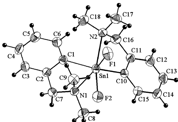
Figure 1. ORTEP representation at 50% probability and atom-numbering scheme for the isomer ( R_{N1}, S_{N2} )- 1b .
