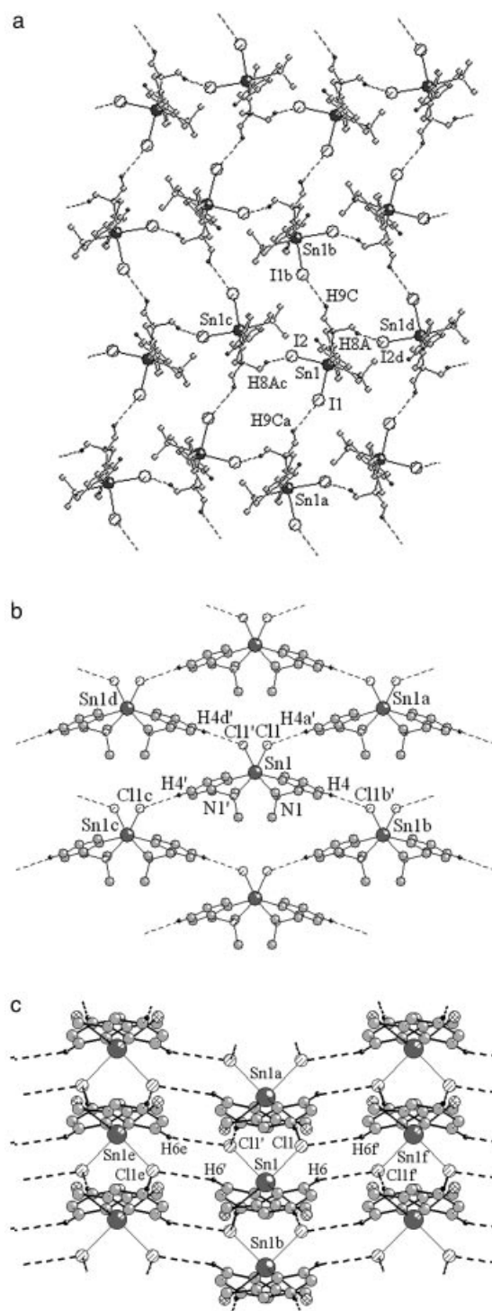
Figure 5. View of supramolecular architectures based on hydrogen bonding (only hydrogen atoms involved in intermolecular interactions are shown): (a) the layer network of ( S_{N1}, S_{N2} ) and ( R_{N1}, R_{N2} ) isomers in the crystal of 1d [symmetry equivalent atoms ( -0.5 + x, 1.5 - y, 0.5 + z ), ( 0.5 + x, 1.5 - y, -0.5 + z ), ( 0.5 - x, -0.5 + y, 1.5 - z ) and ( 0.5 - x, 0.5 + y, 1.5 - z ) are labelled as “a”, “b”, “c” and “d”, respectively]; (b) the layer network of ( S_{N1}, S_{N2} ) isomers in the crystal of 1a [symmetry equivalent atoms ( 0.5 + x, 0.5 + y, z ), ( 0.5 + x, -0.5 + y, z ), ( -0.5 + x, -0.5 + y, z ) and ( -0.5 + x, 0.5 + y, z ) are labelled as “a”, “b”, “c” and “d”, respectively]; (c) 3D supramolecular structure in the crystal of 1a [symmetry equivalent atoms ( -x, 1 - y, 1 - z ) and ( 0.5 - x, 0.5 - y, -z ) are labelled as “e” and “f”, respectively].
