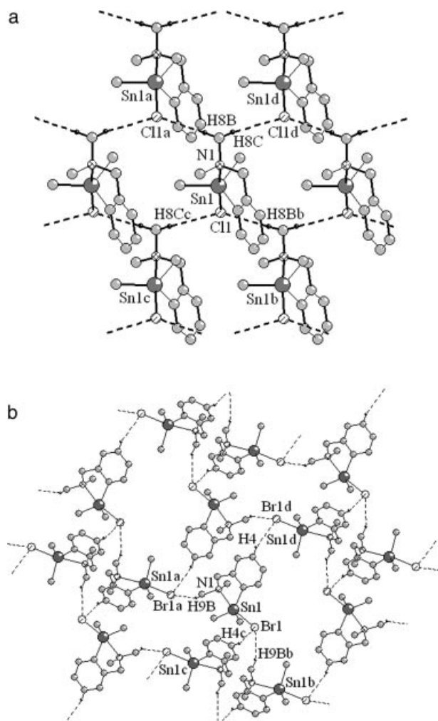
Figure 4. View of the layer network based on intermolecular hydrogen bonds (only hydrogens involved in intermolecular interactions are shown) in the crystals of (a) 2a' [symmetry-equivalent atoms ( 1.5 - x, 0.5 + y, 0.5 + z ), ( 1.5 - x, -0.5 + y, -0.5 + z ), ( 1.5 - x, -0.5 + y, 0.5 + z ) and ( 1.5 - x, 0.5 + y, -0.5 + z ) are labelled “a”, “b”, “c” and “d”, respectively] and (b) 2c [symmetry-equivalent atoms ( -0.5 + x, y, 0.5 - z ), ( 0.5 + x, y, 0.5 - z ), ( 0.5 - x, -y, 0.5 + z ) and ( 0.5 - x, -y, -0.5 + z ) are labelled “a”, “b”, “c” and “d”, respectively].
